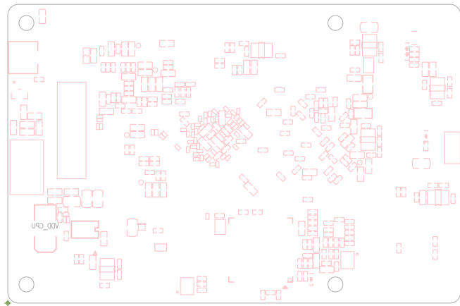
Quartz64 Model-B PCB Placement - silkbottom
