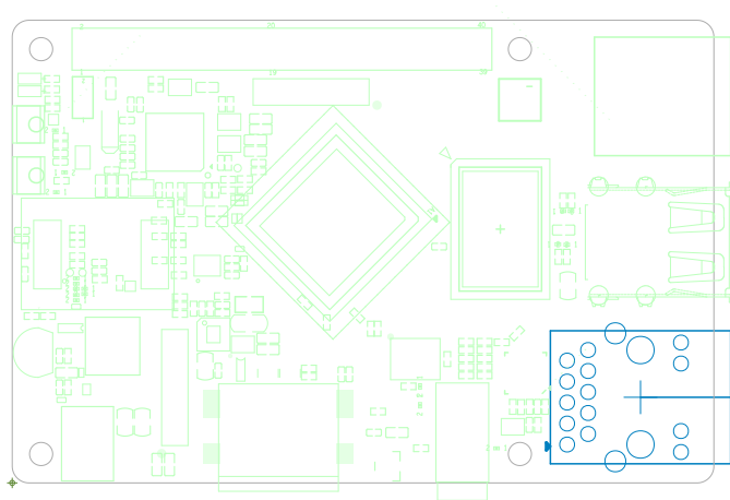
Quartz64 Model B - PCB Placement - silktop
