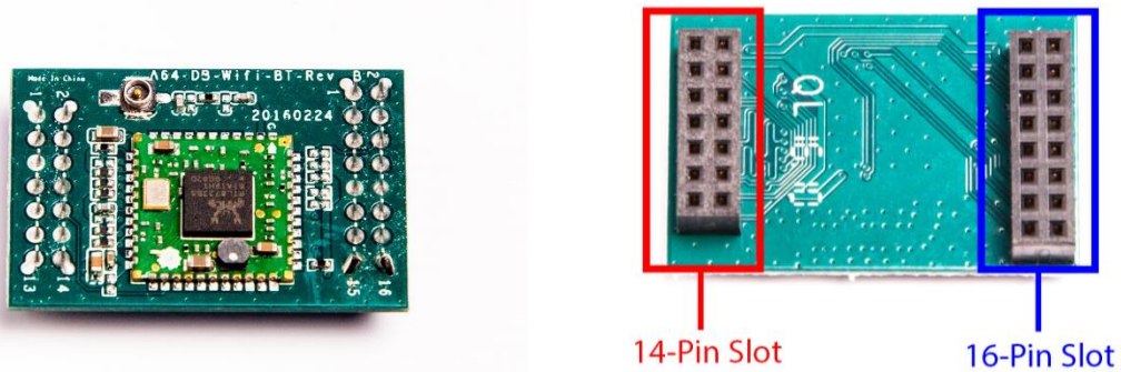
Figure 4: (Left) Top view Wi-Fi/Bluetooth without antenna / (Right) Bottom view (please note the number of pin slots)
