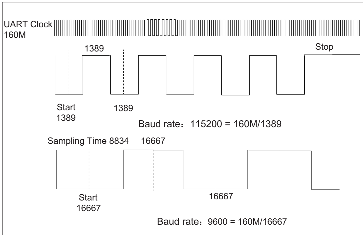
Figure 10.3: UART sample
