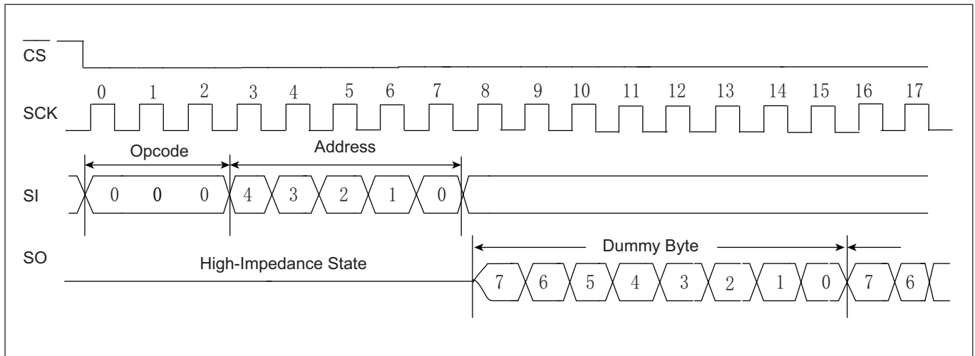
Figure 9.2: SPI ignore
