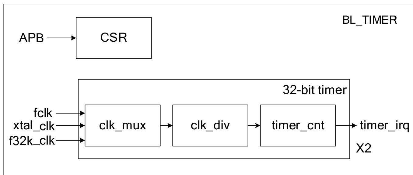
Figure 13.1: Timer block diagram
