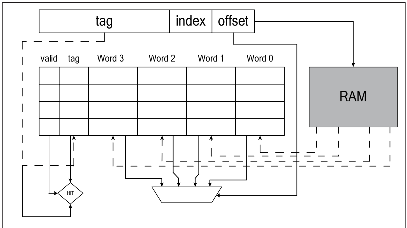
Figure 7.2: Cache architecture
