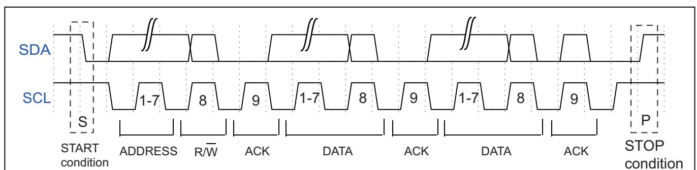
Figure 11.2: Master transmission
