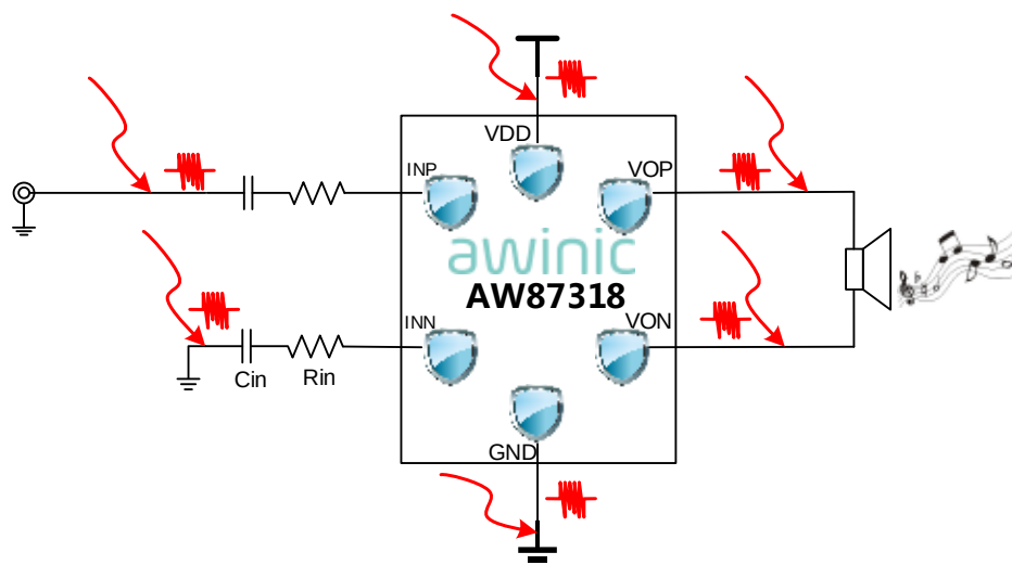
Figure 15 RF Radiation coupling schematic diagram
